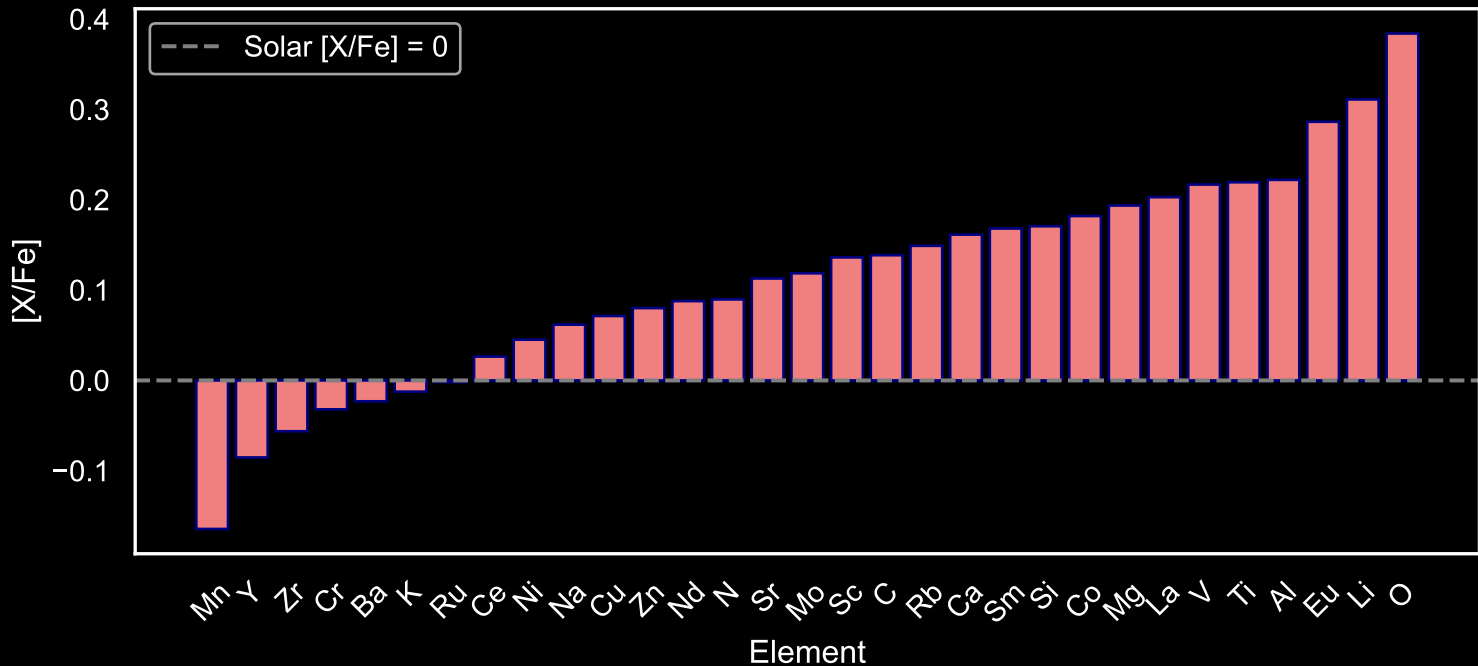
Abundance Pattern for GALAH Red Giants: Star Field [93] (N=81)
