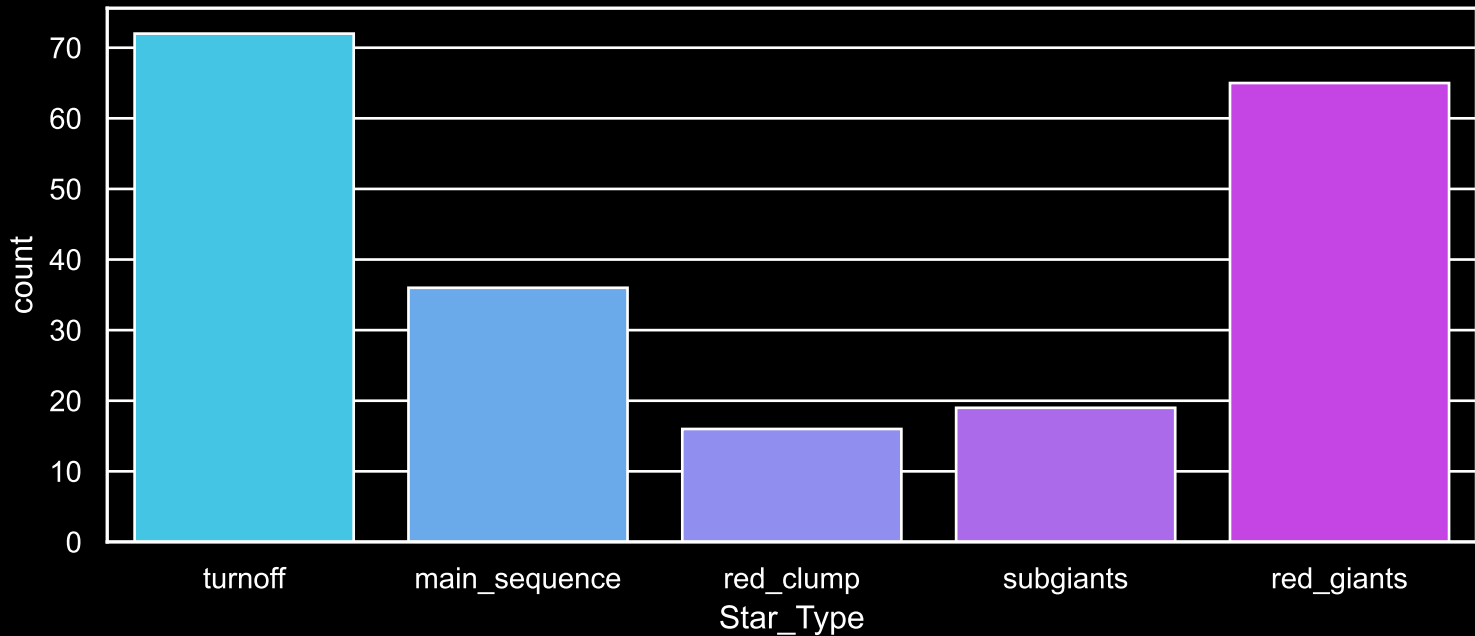
Field [93] Count plot of Star Type
