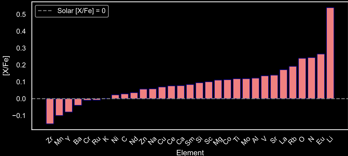
Abundance Pattern for GALAH Star Field [93] (N=208)
