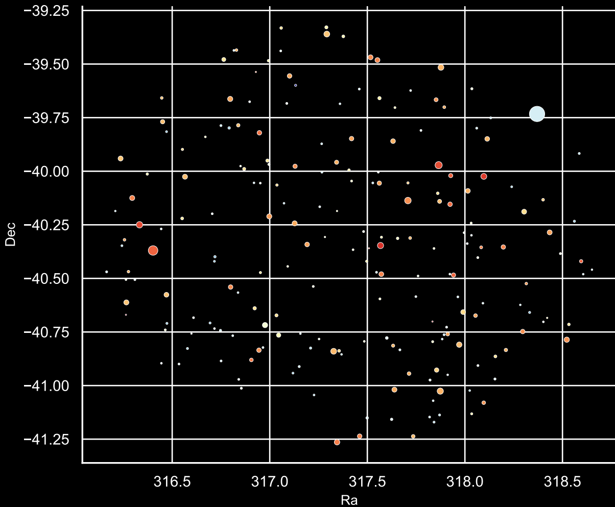
Field [93] Ra [317.4] Dec [-40.35] Stars: 208
