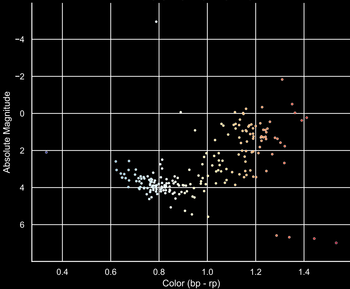
GALAH Hertzsprung-Russell Diagram Field [93] Ra [317.4] Dec [-40.35]
