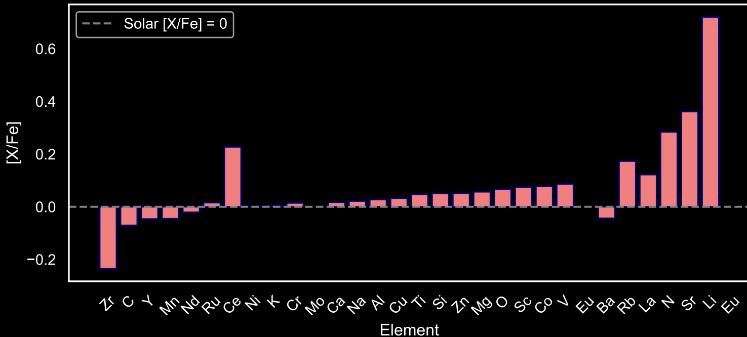
Abundance Pattern for GALAH Main Sequence Stars: Star Field [93] (N=36)
